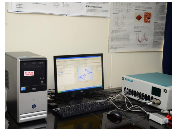
Electrochemical Analyzer
