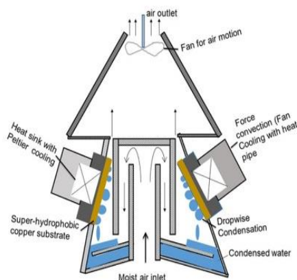
Figure 1: Schematic diagram of proposed atmospheric water generator
