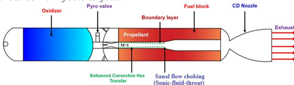
Fig. 1 Illustration of a high-performance hybrid rocket encountering sonic-fluid-throat effect.
