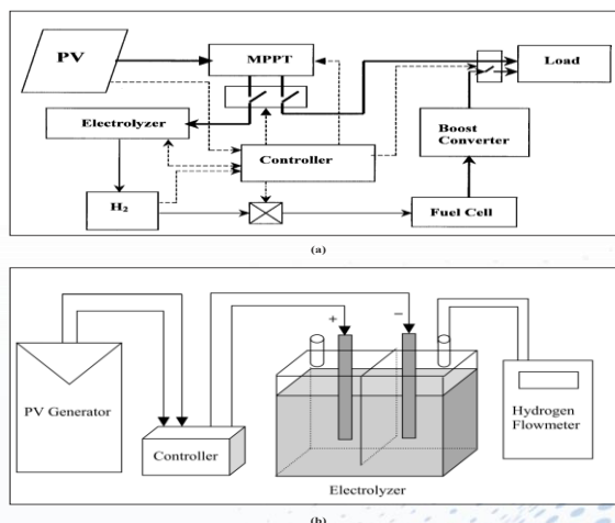
Fig. 1 (a) Line diagram of the project and, (b) Electrolysis Process
