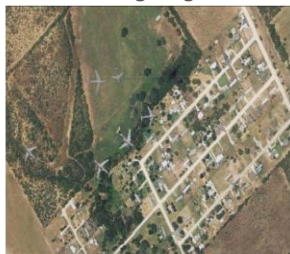
Training Images
