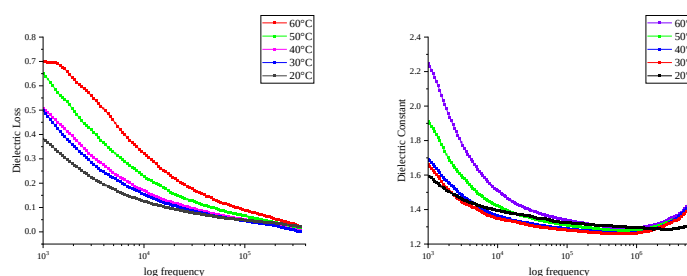
Dielectric permittivity plots of dielectric material (sesame oilseed)
