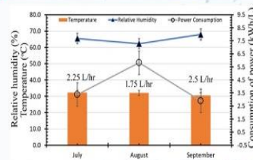
Figure 3: Capacity of water production and Power consumption at various conditions in month of July-September 2023
