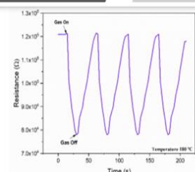
Fig. 7. The change in resistance with time at a temperature of 180 °C in the presence of 1000 ppm of hydrogen gas.
