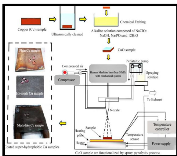
Fig: Schematic diagram for fabrication of various type super-hydrophobic surfaces; (a) plain copper, Hi-mesh surface, and mesh-like surfaces
