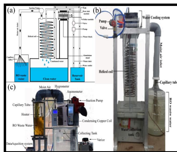
Fig. A device for water recovery from wastewater of household RO systems. (a) Schematic representation of the experimental facility, (b) Photograph of the proposed device and (c) Photograph of the experimental setup for optimizing the parameters of the water recovery device
