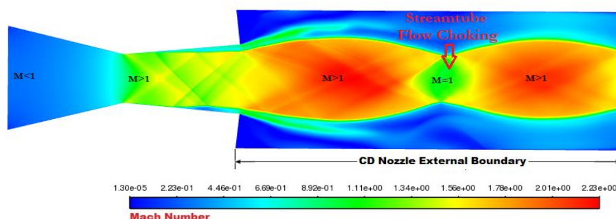
Fig. 2 In silico demonstration of sonic-fluid-throat effect in an external flow.
