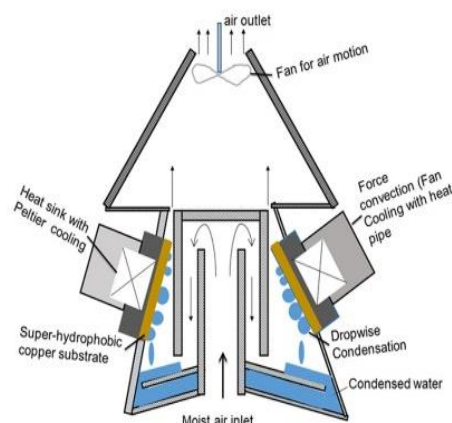
Figure 1: Schematic diagram of proposed atmospheric water generator
