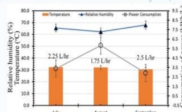
Figure 3: Capacity of water production and Power consumption at various conditions in month of July-September 2023
