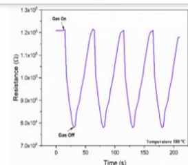
Fig. 7. The change in resistance with time at a temperature of 180 °C in the presence of 1000 ppm hydrogen gas.
