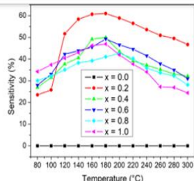
Fig. 5. Sensitivity (%) of the sensors with the temperature range from 80 to 300 °C in the presence of 1000 ppm of H 2 concentration.
