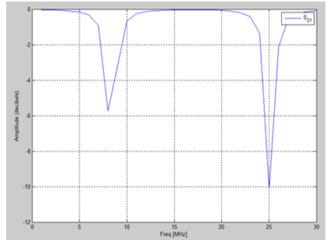
Fig.7: Amplitude spectrum of the transfer function when the length is increased
