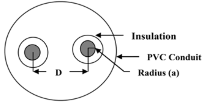
Fig.4: Approximate model of indoor power line
