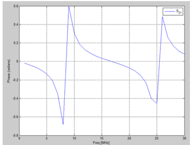
Fig.8: Phase spectrum of the transfer function when the length is increased
