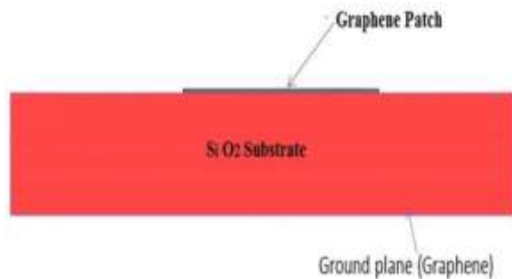
Fig. 5. Graphene Patch Antenna Cross Sectional View
