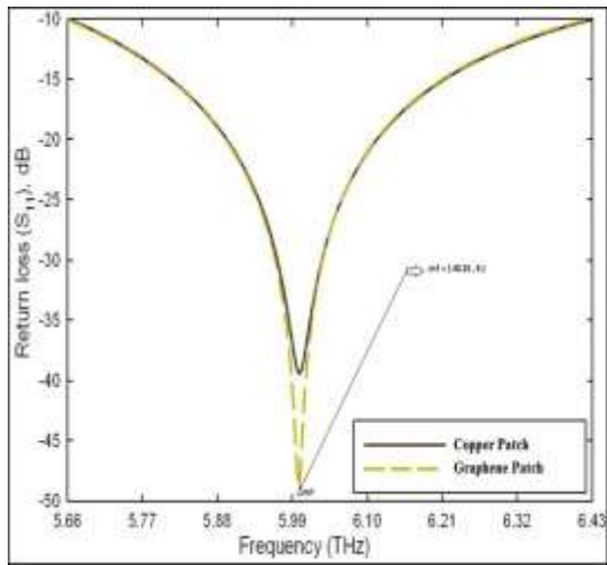
Fig. 6. Return Loss Comparative Graph of Copper and Graphene Patch Parameters
