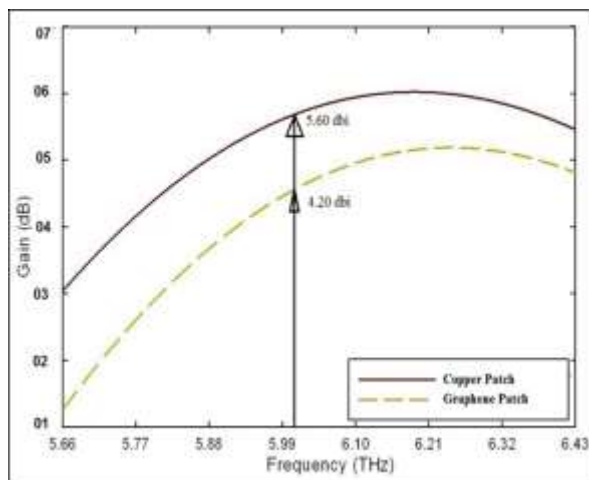
Fig. 8. Gain with Copper Patch and with Graphene Patches
