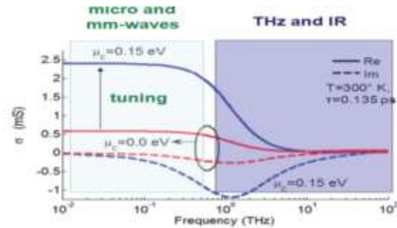
Fig. 2. Surface Conductivity Curve Microwave and Terahertz waves
