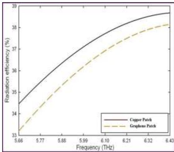
Fig. 7. Radiation Efficiency of Patch Antenna With Copper and Graphene as a Patch Material
