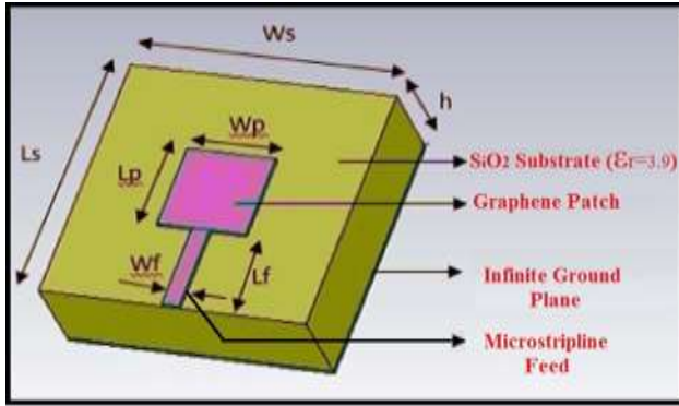
Fig. 1. GMPA (Graphene Microstrip patch Antenna)
