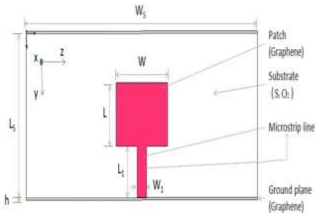
Fig. 4. Graphene Patch Antenna Design with Microstrip line Feeding
