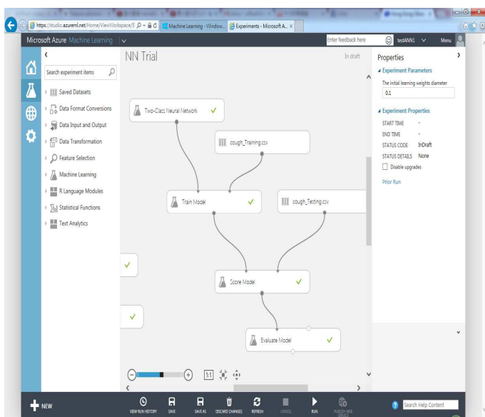
Fig. 2. The model is constructed in the Machine Learning Studio
