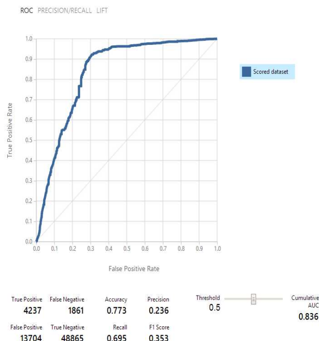
Fig. 6. The True Positive Rate vs the False Positive Rate
